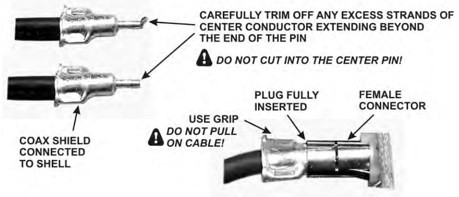
Figure 83. TMP Cable Connectors.
