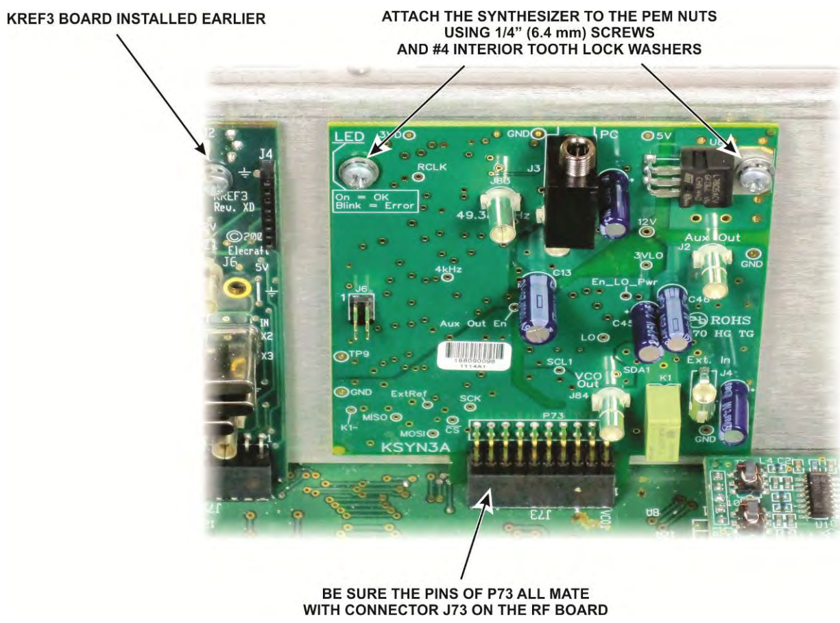
Figure 82. Installing the KSYN3 Board.
