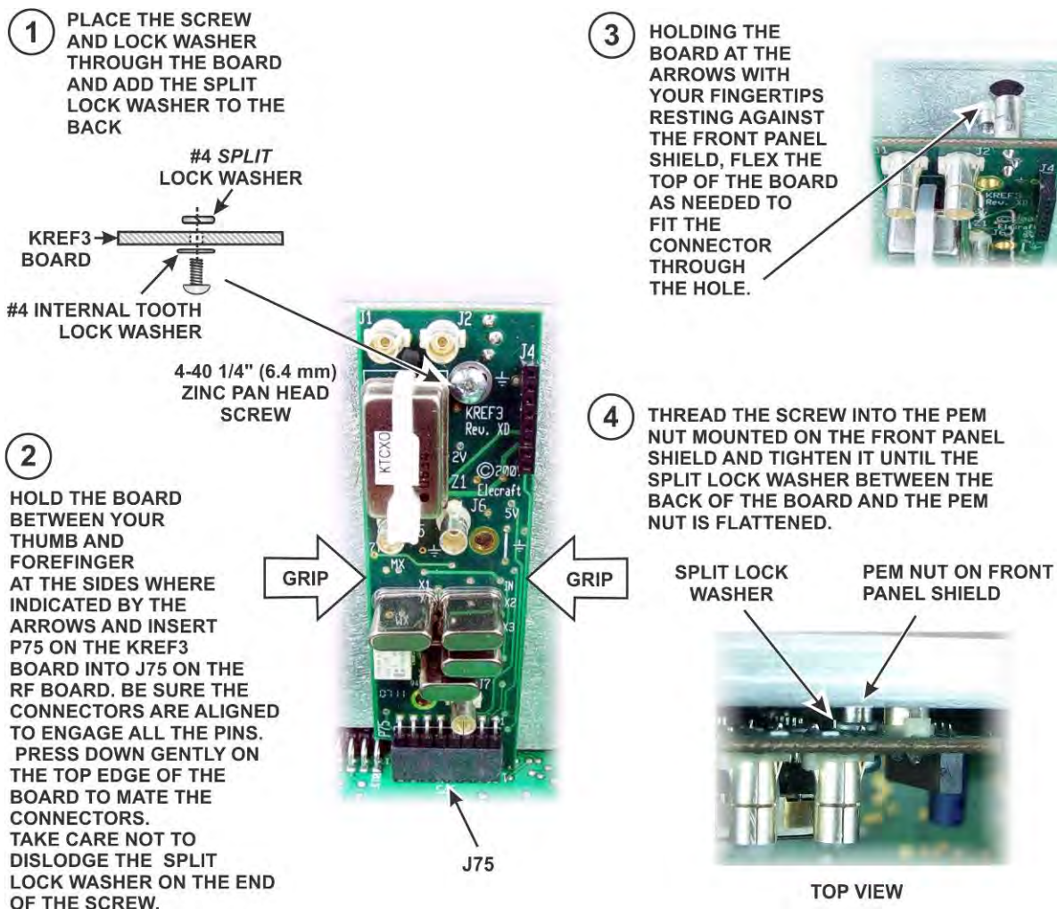
Figure 80. Installing KREF3 Board.
