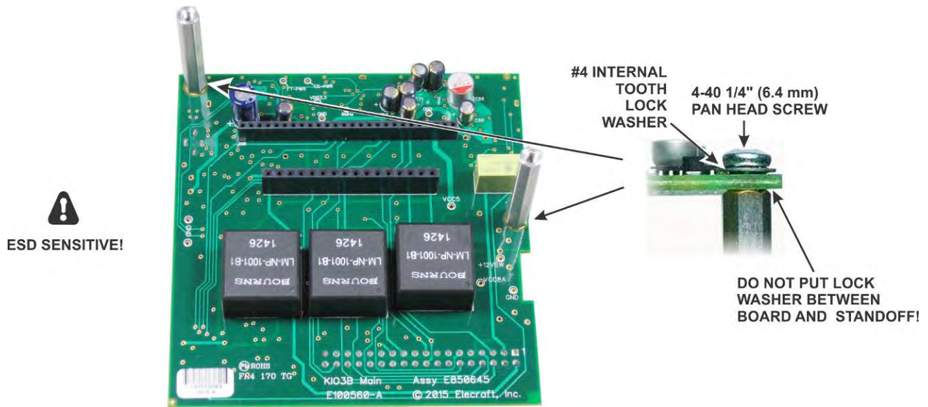
Figure 56. Mounting Standoffs on the KIO3B Main Board.
