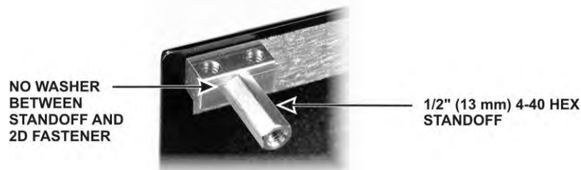
Figure 73. KAT3A/KANT3A Mounting Standoff.
