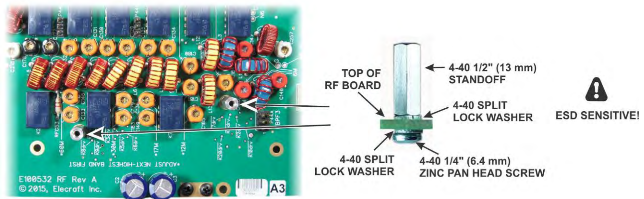
Figure 35. Installing KBPF3A Standoffs.
