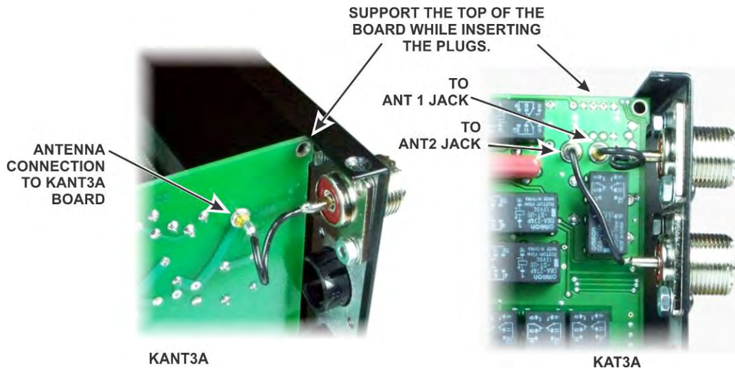
Figure 70. ANT Connections to KANT3A or KAT3A Boards.
