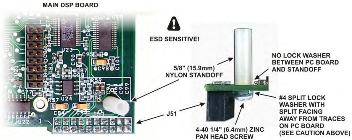
Figure 27. Installing the Nylon Standoff.
