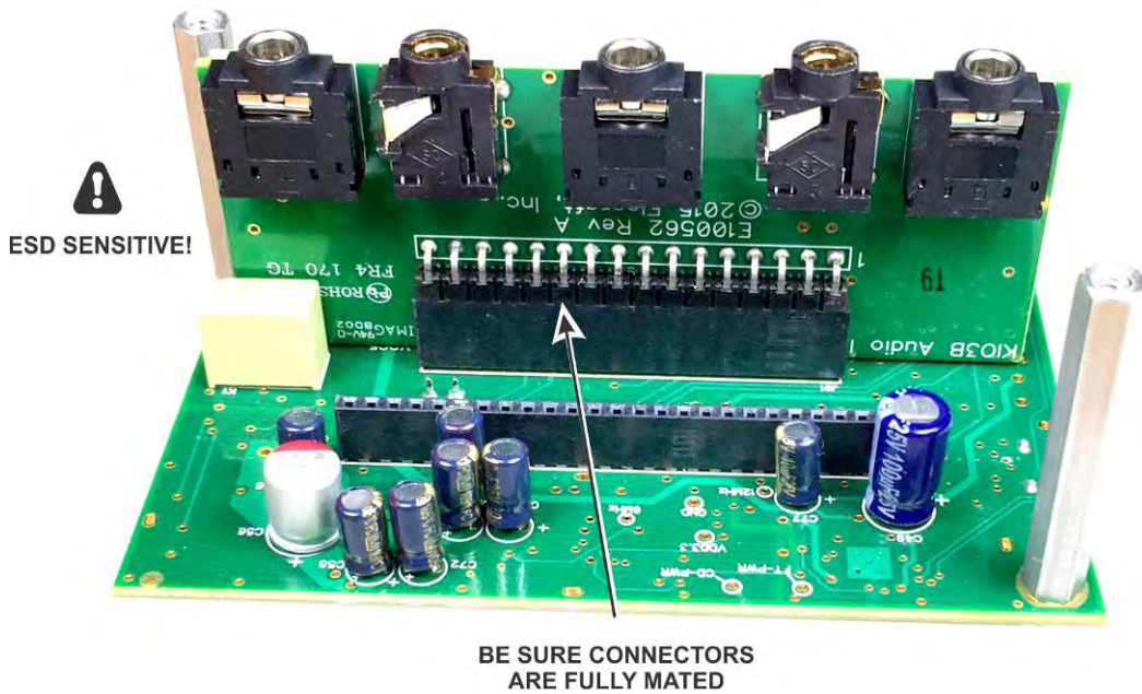
Figure 57. Mounting Audio I/O Daughter Board on KIO3B.
