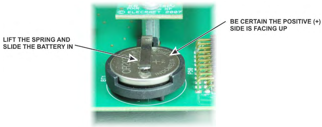
Figure 62. Installing BT1.
