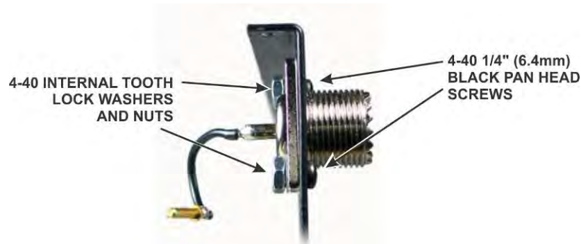
Figure 44. Mounting the ANT1 Connector.
